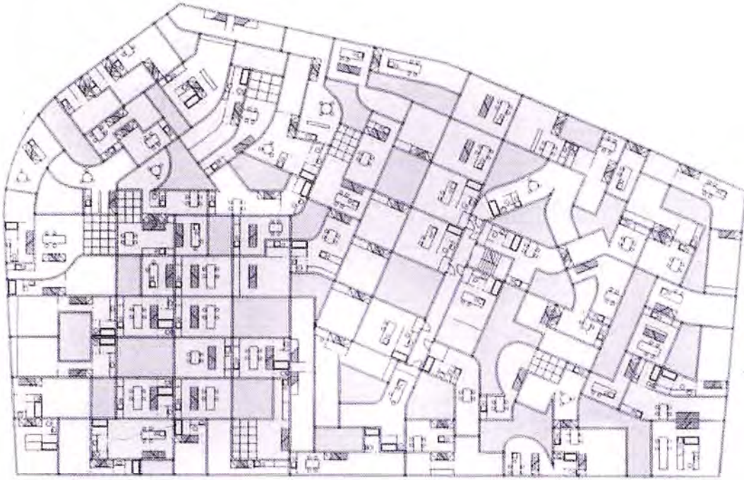
Pazo de Aguiar / Second floor plan
