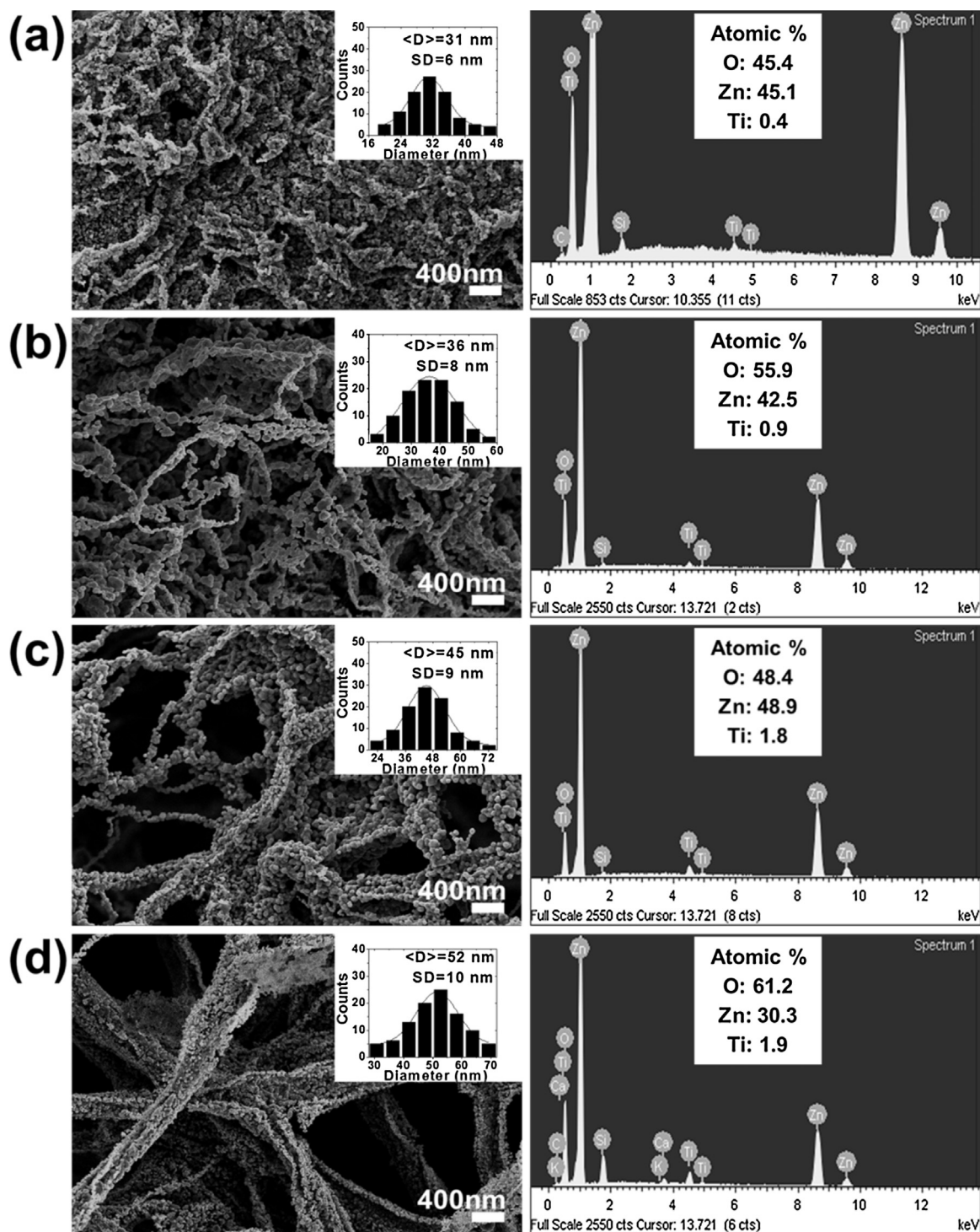
Fig. 4. FE-SEM images (left sides) and EDS spectra (right side) of the ZnO/TiO 2 nanostructures obtained by calcination of the precursor fibers prepared using the spinning solutions with different ZnAc-to-PVA ratios: (a) 1:2, (b) 2:3, (c) 1:1, and (d) 3:2. The nanoparticle distributions with corresponding standard deviations (SD) are shown as insets.
