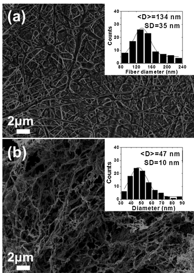
Fig. 2. FE-SEM images of the precursor fibers fabricated using the spinning solution with a ZnAc-to-PVA ratio of 2:3 before (a) and after (b) calcination at 600 °C. The diameter distributions with corresponding standard deviations (SD) of the fabricated precursor fibers (a) and the mean diameter of the final ZnO skeleton nanostructures (b) are shown as insets.
