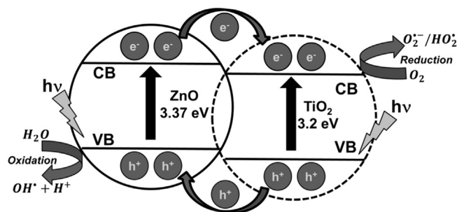
Fig. 8. A schematic diagram illustrating the principle of charge separation and photocatalytic activity of the ZnO/TiO 2 composite nanostructures system.
